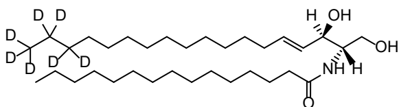
15:0-18:1(d7) Cer
