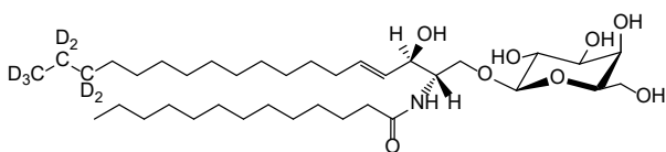
13:0-18:1(d7) GalCer
